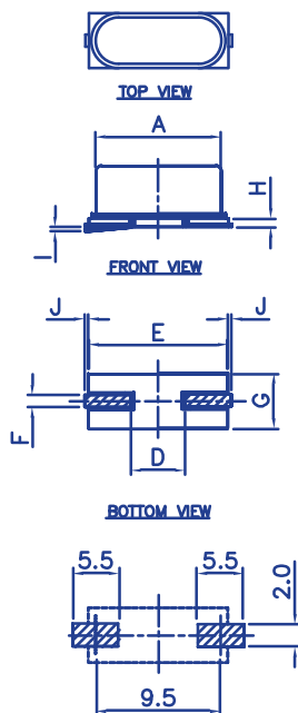
RECOMMENDED LAND PATTERN
