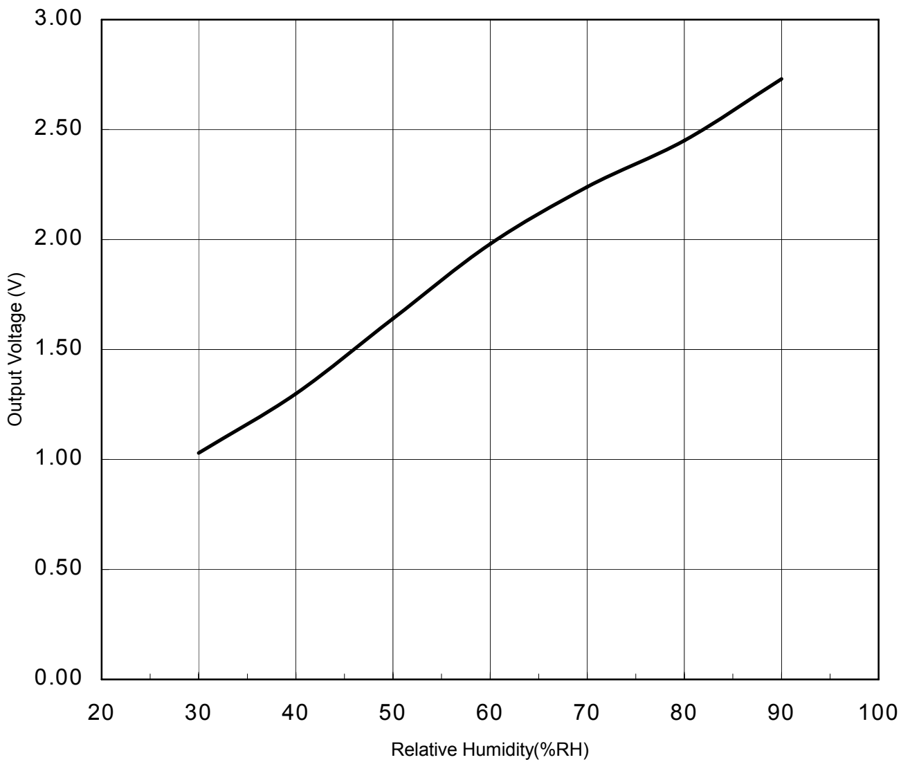
Humidity Output 0~3.3V characteristics
