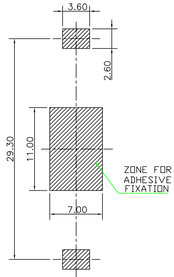
PCB LAYOUT
