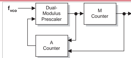
Figure 3: Feedback Divider
