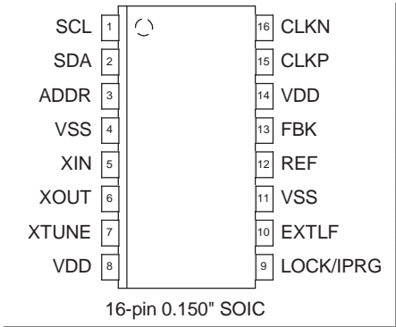
Figure 1: Pin Configuration
