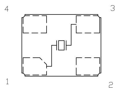
INTERNAL CONNECTION
