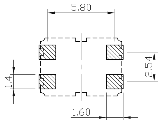
RECOMMENDED LAND PATTREN
