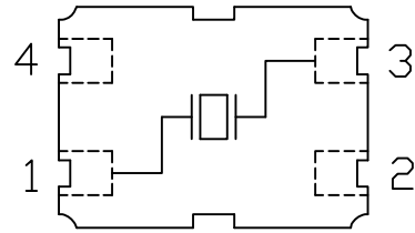
INTERNAL CONNECTION
