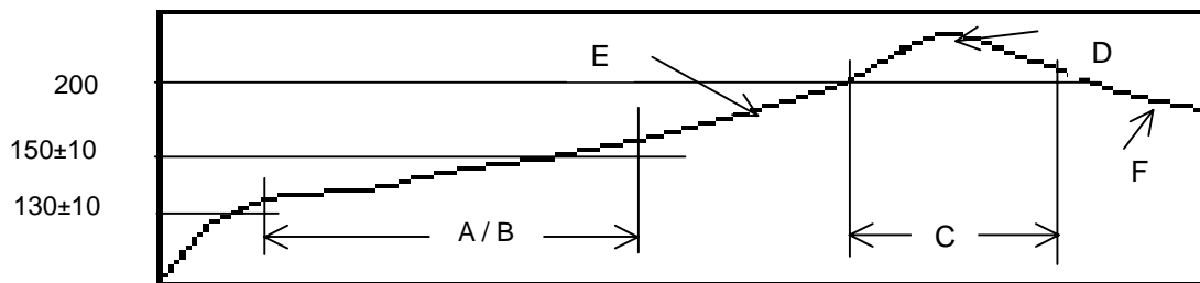
SOLDER TEMPERATURE PROFILE ( Reflow Soldering )
